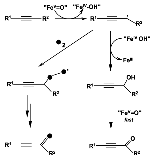
Scheme 2 Proposed mechanism for alkyne oxidation.
