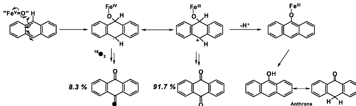
Scheme 1 Proposed mechanism of anthracene oxidation. “Fe V =O” stands for FePcS-based species having two redox equivalents above the Fe III state.
